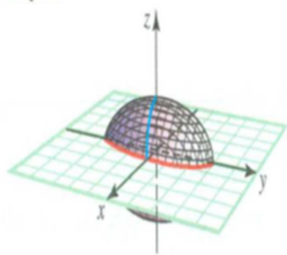
Ellipsoid
