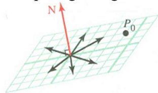
Figure 9.58 A plane through P with a normal vector N
