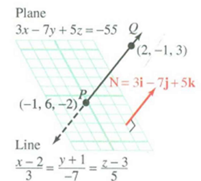
Figure 9.60 Graph of a plane
