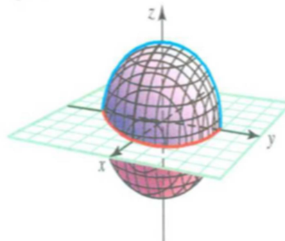
Sphere
